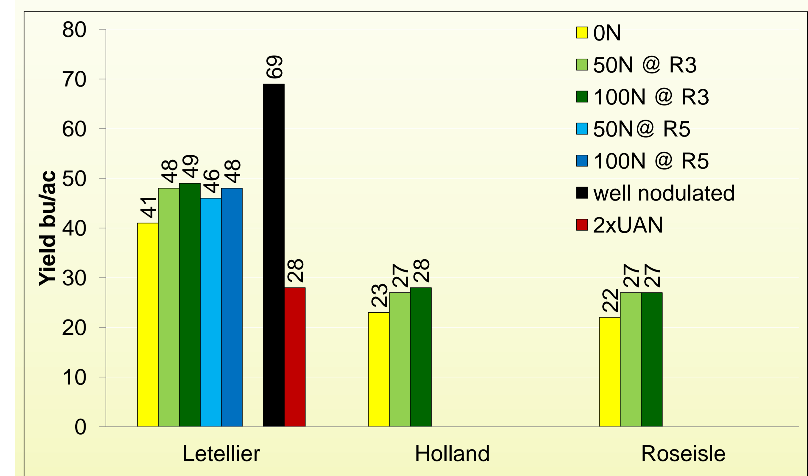
Figure 7. Soybean yield response to rescue N applications.
